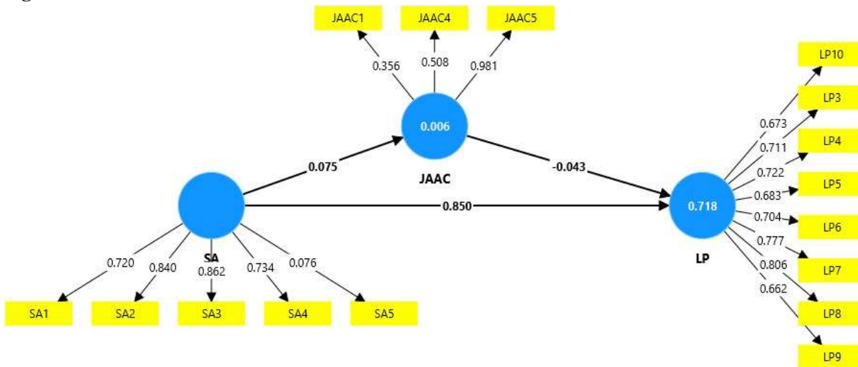
Fig 1: Measurement Model
